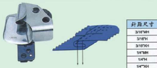
JZ-15525 35800(F337) 弹弓嘴迂仁埋夹 Sprig Type Side Seam Folder-Union Special Type
