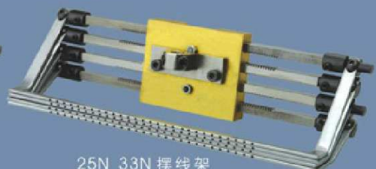
25N 33N 摆线架 JZ-12119
